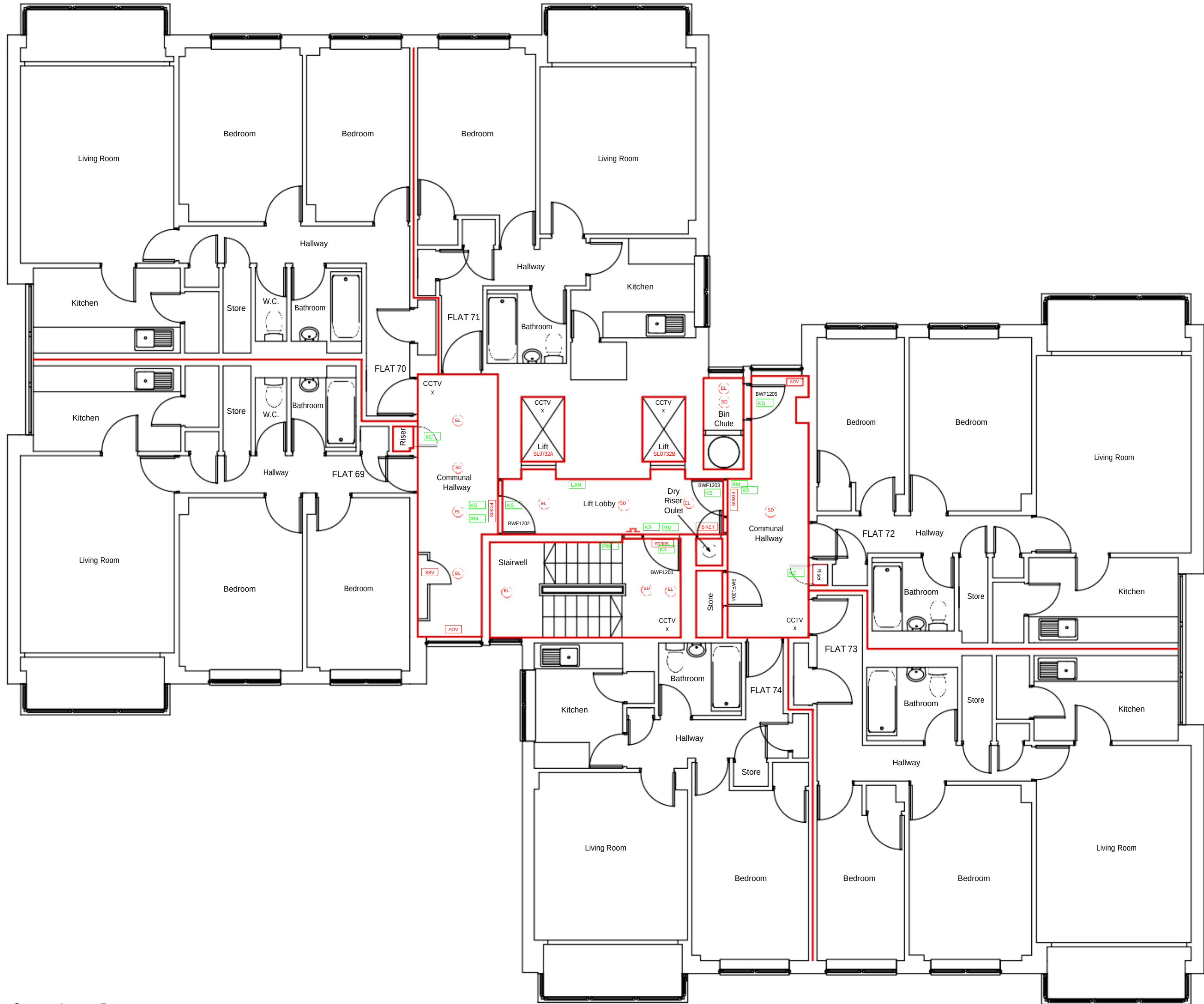
TWELFTH FLOOR
